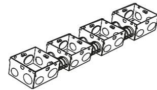
4 Gang BS GI Box
